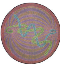
Electromagnetism
